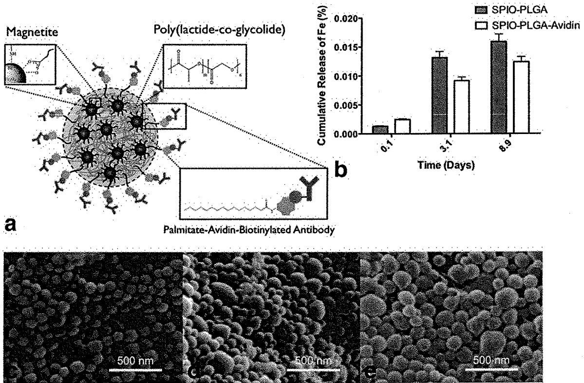
FIG. 2. a: Schematic of SPIO-loaded PLGA nanoparticles with incorporated Avidin surface functionality for conjugating biotinylated antibodies. b: Inductively couple plasma mass spectrometer determination of negligible Fe release from PLGA nanoparticles in PBS at 37°C. Field-emission scanning electron microscopy of (c) blank PLGA nanoparticles, (d) SPIO-loaded PLGA nanoparticles, and (e) SPIO-loaded PLGA nanoparticles with Avidin surface functionality, respectively.
