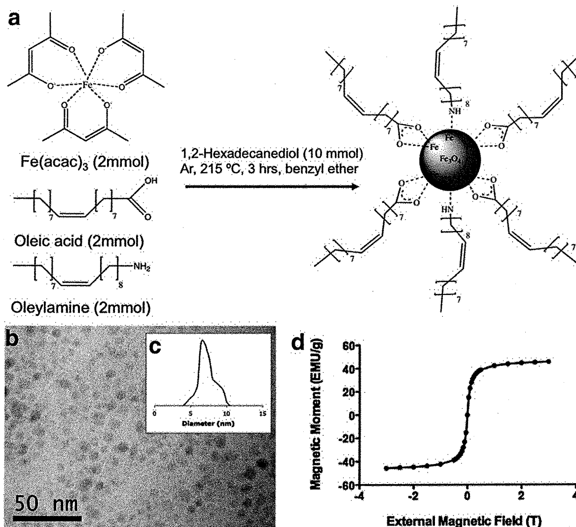
FIG. 1. a: Synthesis of hydrophobic SPIO nanoparticles through high temperature reduction of \text{Fe}(\text{acac})_3 . b: TEM shows discrete nanoparticles with (c) average diameter being \sim 7 nm in diameter. d: SQUID shows SPIO nanoparticles with the absence of magnetic hysteresis.
